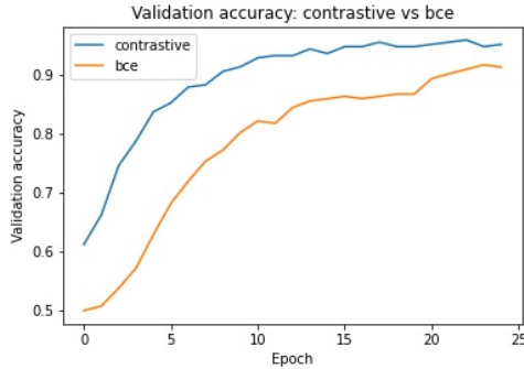
Fig. 5. Validation accuracy through training (bce = binary cross-entropy)
