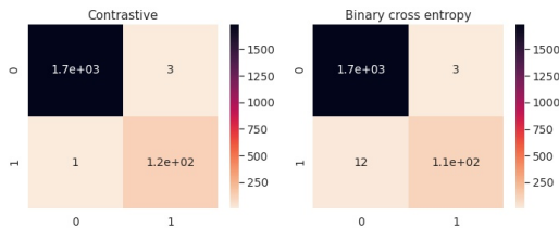
Fig. 6. Confusion matrix of our model (left) and original code clone detection model (right)
