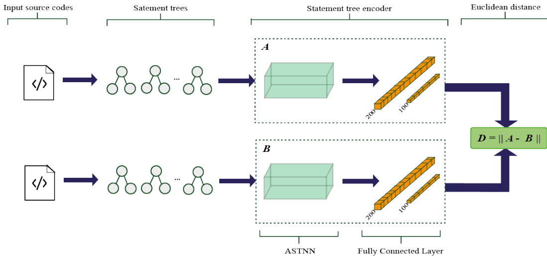
Fig. 4. Code clone detection framework. Each input source code is transformed into a set of tree data structures called statement trees as in Fig. 1, then, these sets are passed into the same statement tree encoder which outputs a 100-D vector for each input source code. The Euclidean distance between the vectors is then calculated and pass to the contrastive loss function.
