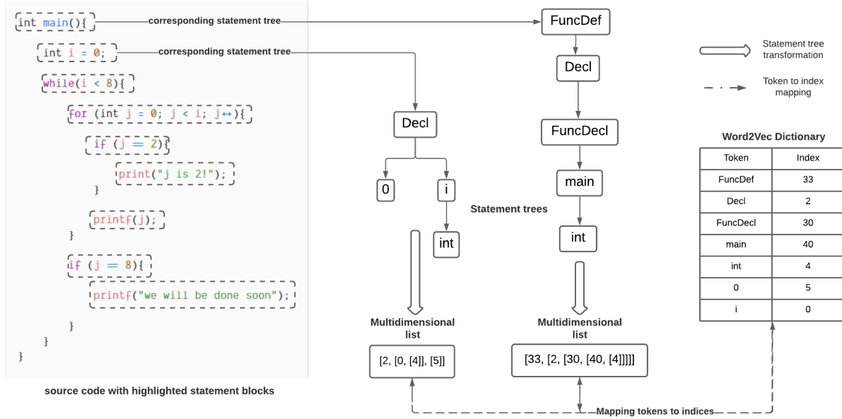
Fig. 2. Preprocessing framework of the input source codes. The statement nodes (framed in rectangles with dotted borders) are extracted into their corresponding statement tree then, these statement trees are transformed into a multidimensional list where the tokens (Decl, FuncDef, main, int, etc.) are replaced by their indexes from a Word2Vec model which has been trained with these tokens.
