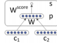
Fig. 1. Recursive layer with a parent node p and two children nodes, c_1, c_2
