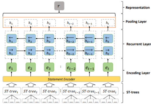
Fig. 3. Proposed architecture of the AST Neural Network for source code representation [1].
